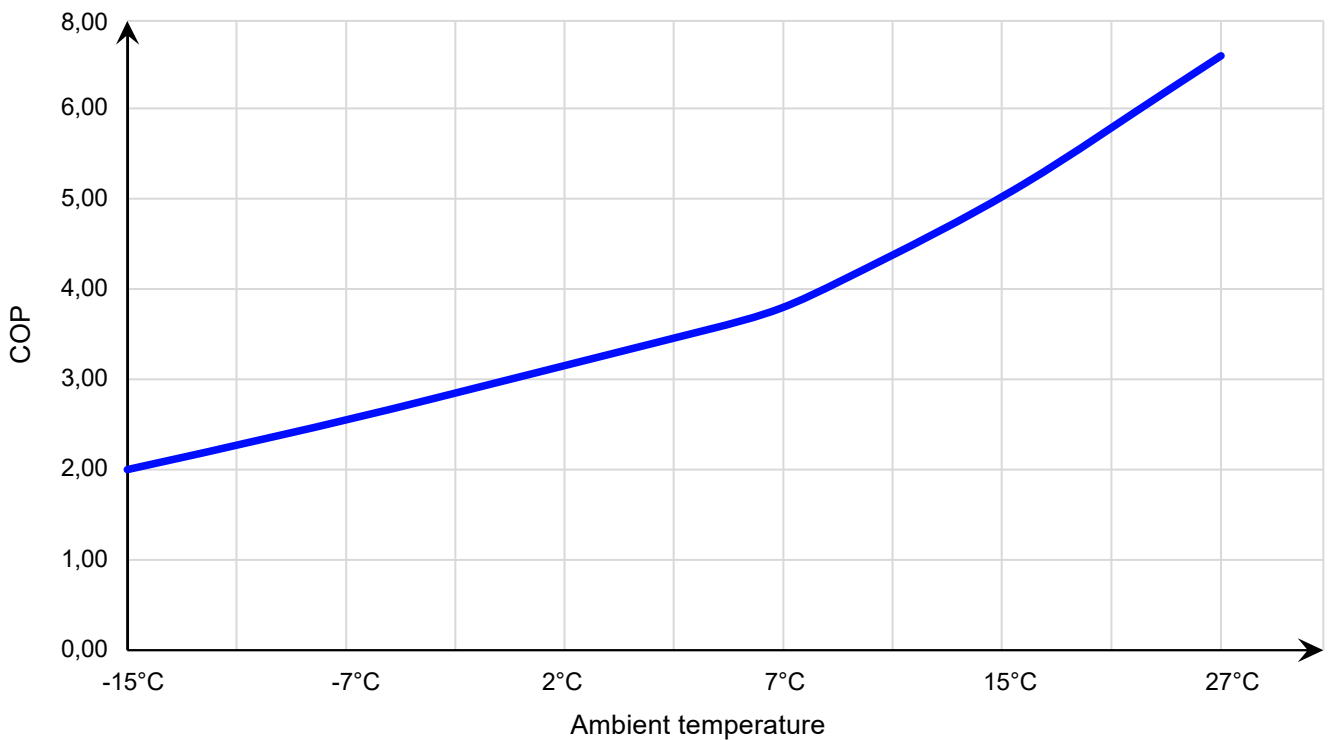
34-180630 COP Curve
